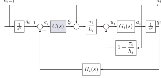
Fig. 3. Block diagram of controller (11) with PD implementation (13).
