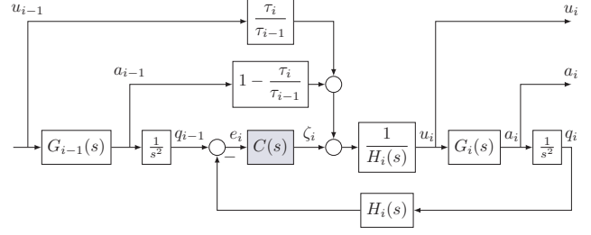
Fig. 2. Block diagram of controller (6).
