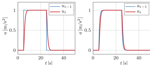
Fig. 9. Time response of controller (11), (16) in a heterogeneous setting ( \tau_i = 0.1 , \tau_{i-1} = 0.6 ).
